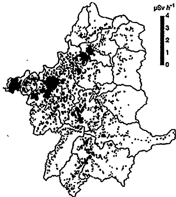
d) 7th Airborne survey and Glass Badge (2013/7-9)
