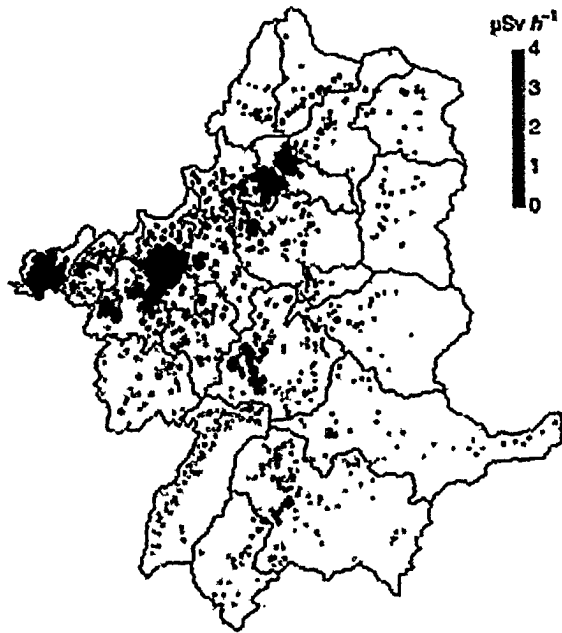
a) 4th Airborne survey and Glass Badge (2011/9-11)
