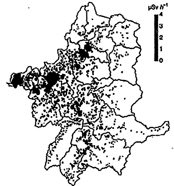
f) 9th Airborne survey and Glass Badge (2014/10-12)
