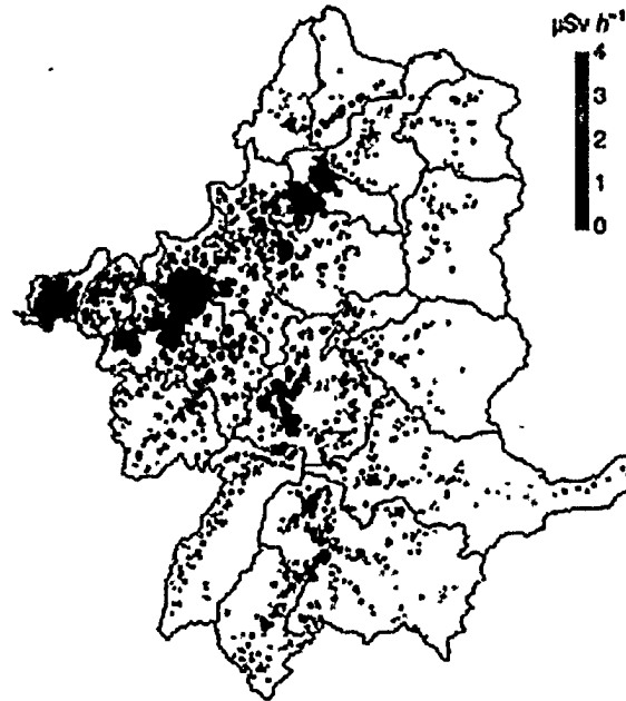
e) 8th Airborne survey and Glass Badge (2013/10-12)
