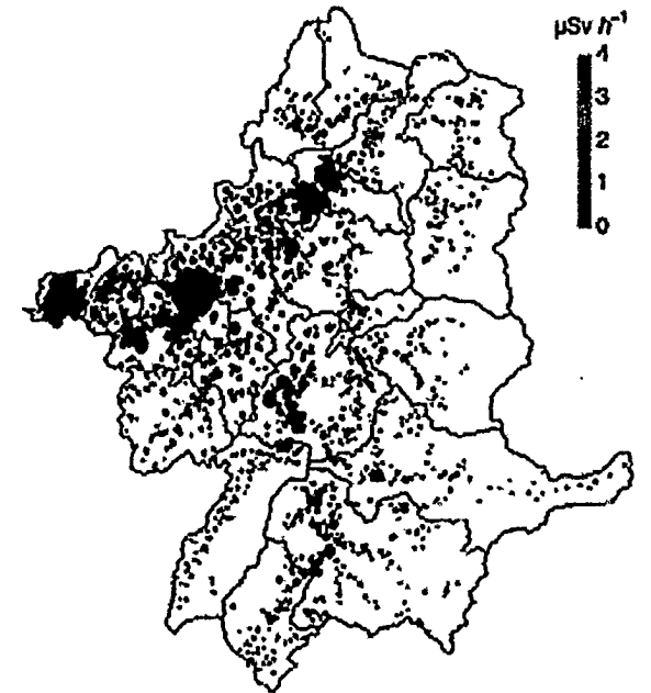
c) 6th Airborne survey and Glass Badge (2012/10-12)
